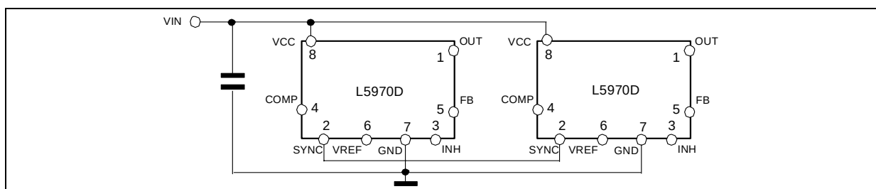
Figure 19. Synchronization example
