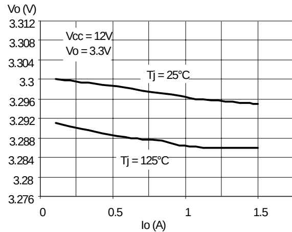
Figure 5. Line Regulation
