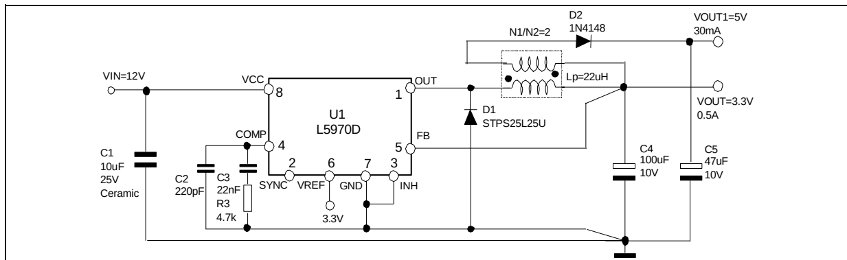
Figure 16. Dual output voltage with auxiliary winding
